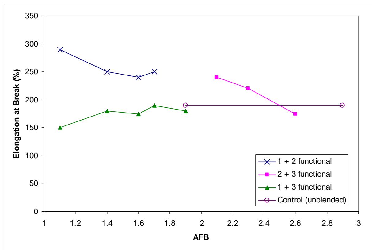
Figure 2. Elongation at break for gasket prototypes with varying AFB.
