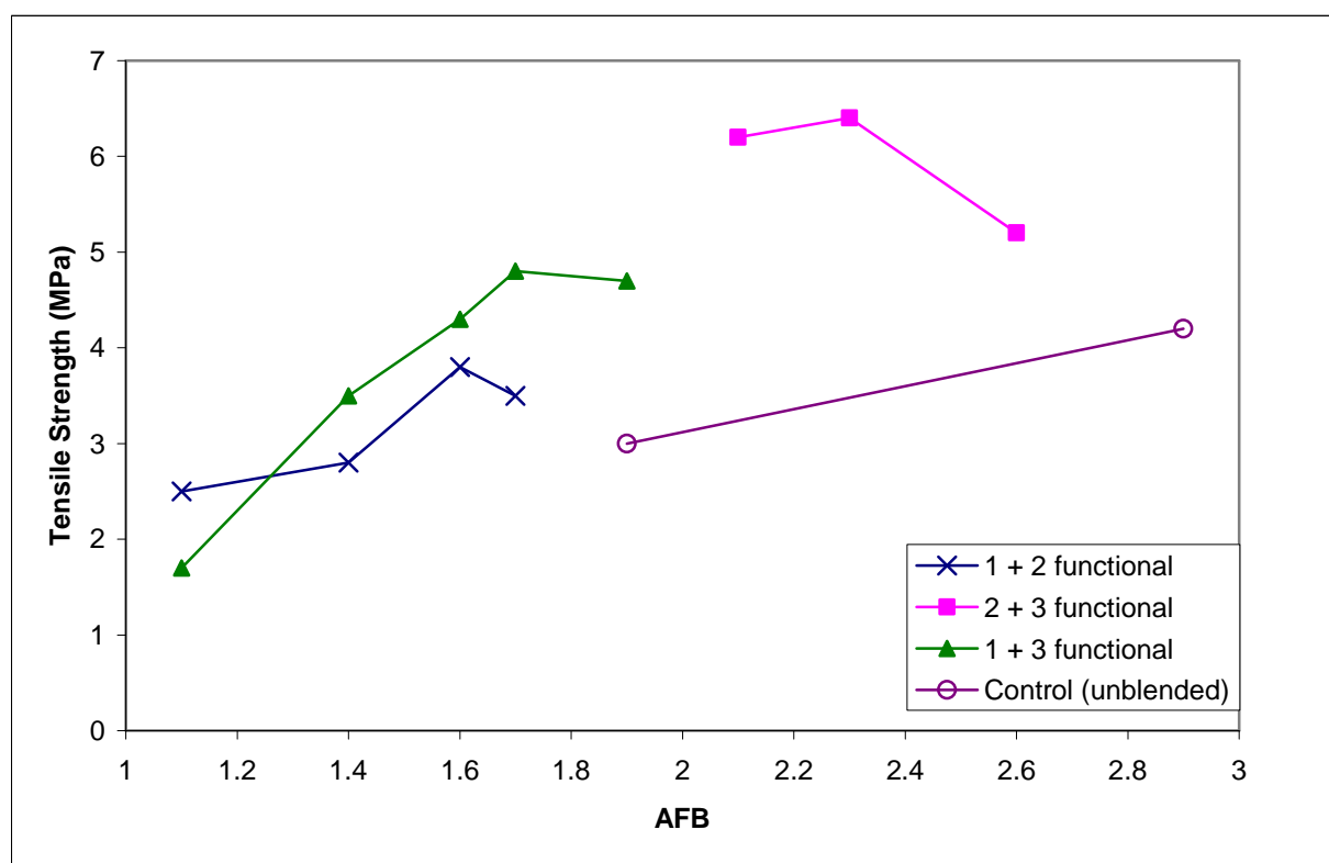
Figure 1. Tensile strength for gaskets with different AFB.
